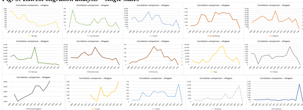
Fig. 3: Extrem migration analysis – single states
