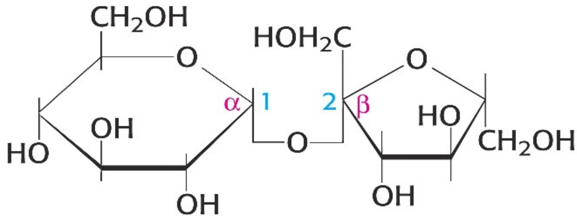
Sucrose
