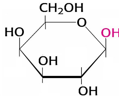
\beta -D-Galactopyranose
