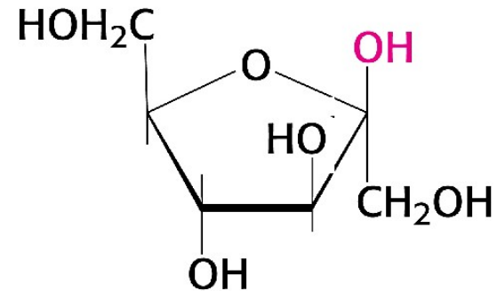
β-D-Fructofuranose
