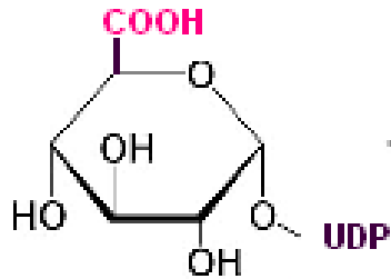
UDP-glucuronic acid
