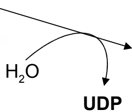
UDP-glucuronic acid
