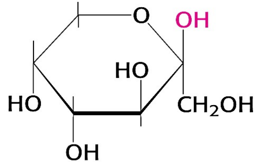
β-D-Fructopyranose
