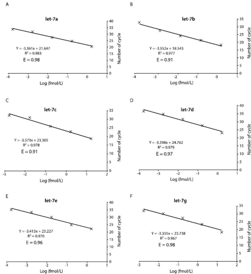
FIGURE 1. Absolute standard curves for let-7a (A), let-7b (B), let-7c (C), let-7d (D), let-7e (E) and let-7g (F) used for calculation of let-7 miRNAs concentrations (fmol/L) in the urine samples. E - qPCR reaction efficiency.
