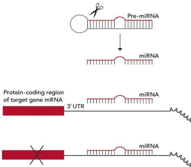
Fig. 11. Schematic representation of miRNA function.
