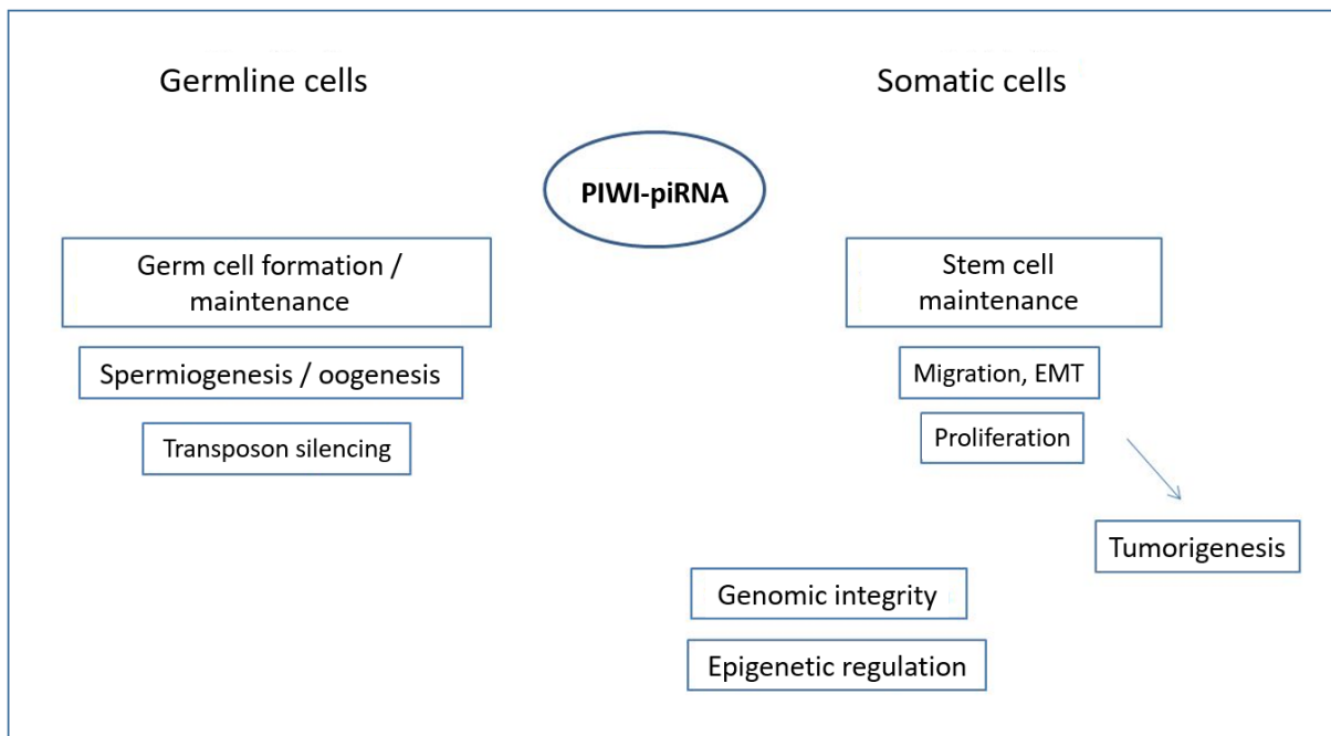
Fig. 12. Schematic representation of the cellular functions of PIWI-piRNA. Adapted from Litwin et al. (45).
