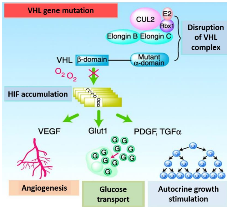
Fig. 9. VHL/HIF pathway. Adapted from Bratslavsky et al. (9).
