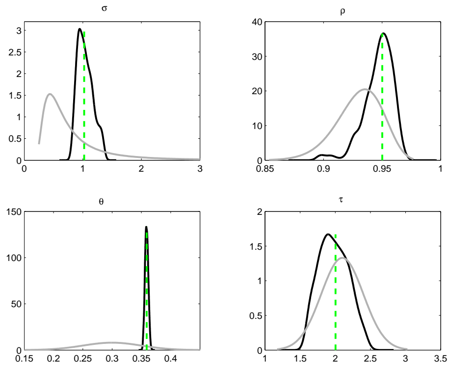
Figure 3: Posterior.
