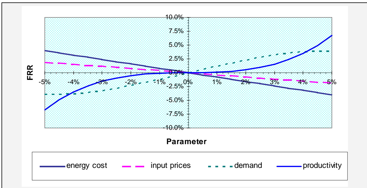
Figure 2.5 Sensitivity analysis
