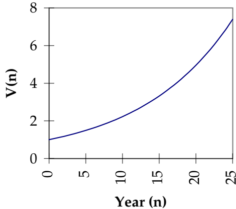
Figure 1.1: Exponential Growth
