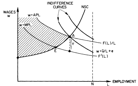
FIGURE 4. SOCIAL OPTIMUM AT A
