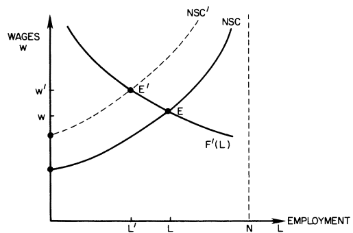
FIGURE 3. COMPARATIVE STATICS
