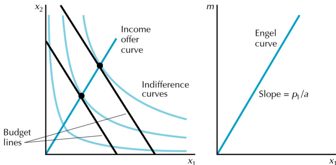
A Income offer curve
