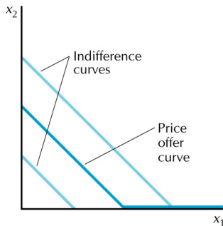
A Price offer curve
