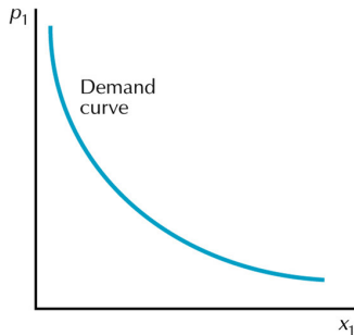
B Demand curve
