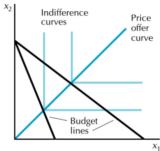
A Price offer curve
