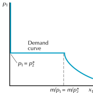
B Demand curve
