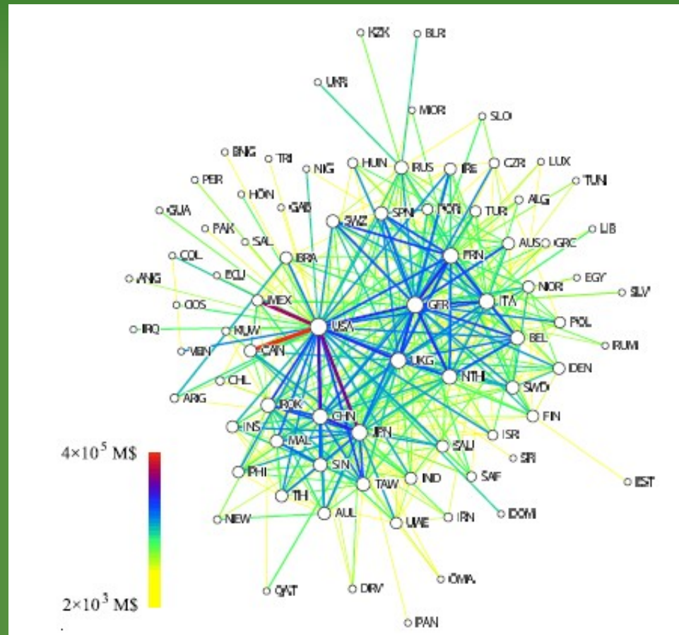
FIG. 1: (Color online) A subnetwork of the ITN for the year 2000, where only links with the highest 4 % of weights and the associated nodes (countries) are included [20], yielding in total 80 nodes and 411 links. The node size is proportional to its strength and link color to its weight. Link weights are defined as the volume of annual trade between two countries in M\$ .
