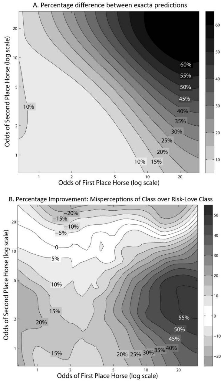
FIG. 4.—Differences between theories
