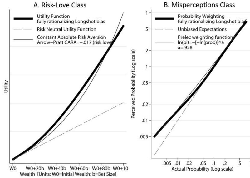
FIG. 3.—The win data are completely rationalized by both classes
