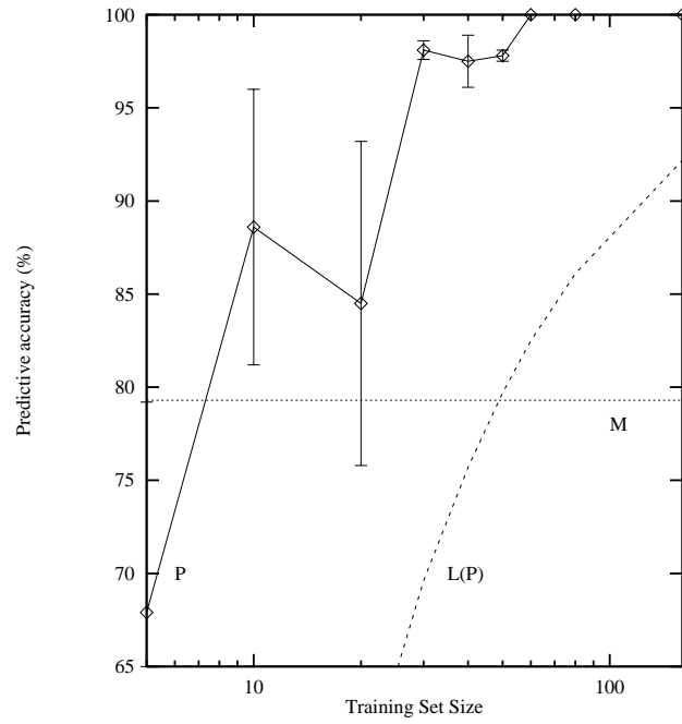
Figure 5: Predictive accuracy versus bound for animal taxonomy
