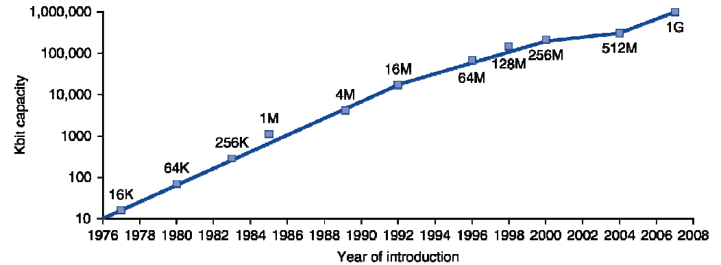
DRAM capacity
