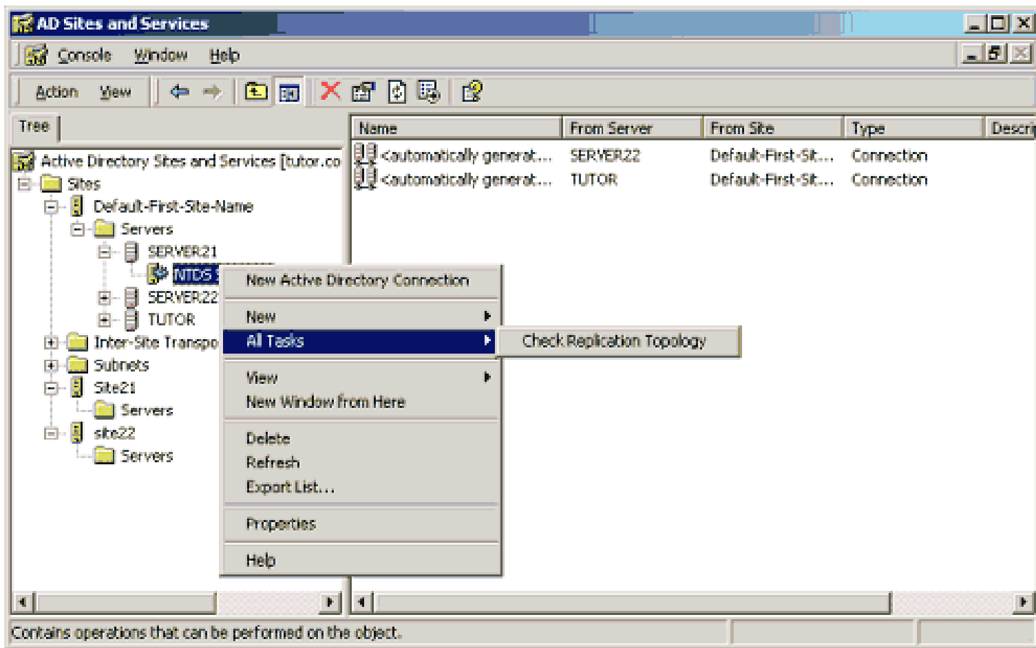
Figure 6.– Manually checking the replication topology
