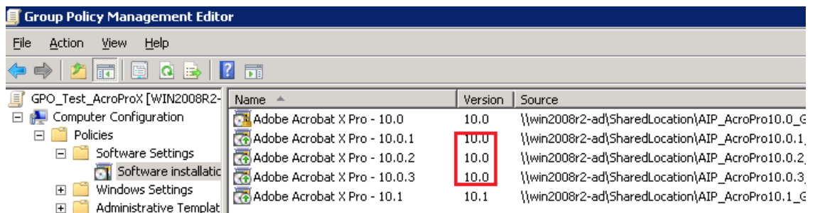
Figure 6 GPO summary
