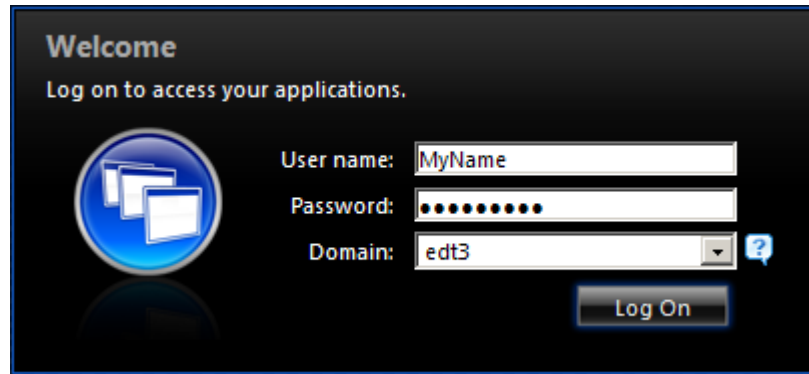
Figure 1 Citrix: Authentication
