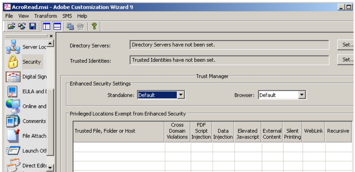
Figure 4 Customization wizard
