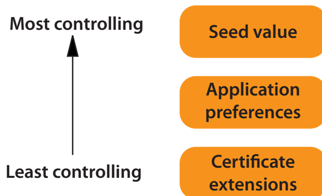
Figure 3 Precedence order
