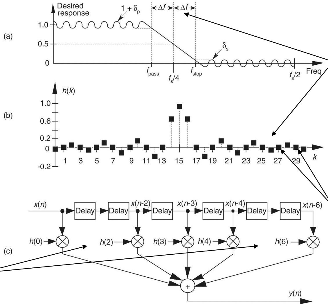
Figure 5-33 Half-band FIR filter: (a) frequency magnitude response (transition region centered at f_s/4 ); (b) 31-tap filter coefficients; (c) 7-tap half-band filter structure.
