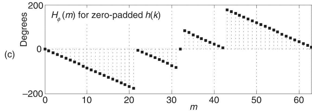
Figure 5-48 High-resolution FIR filter frequency response: (a) zero-padded h(k) ; (b) discrete magnitude response; (c) phase response.
