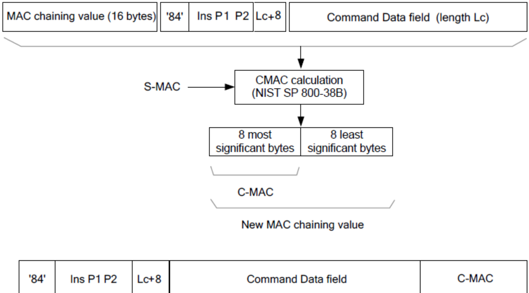
Figure 6-1: APDU C-MAC Generation
