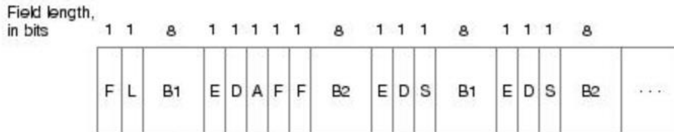
TE frame (terminal to network)
