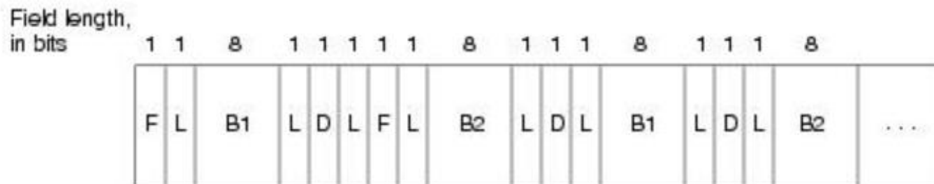
NT frame (network to terminal)
