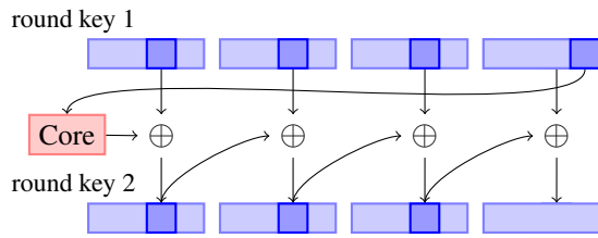
Figure 6: In the 128-bit AES key schedule, three bytes of each round key are entirely determined by four bytes of the preceding round key.
