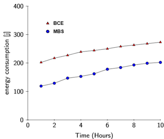
Fig. 4 Energy consumption
