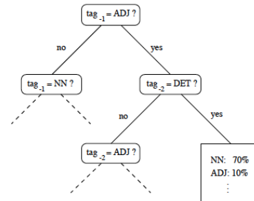
Figure 1: A sample decision tree
