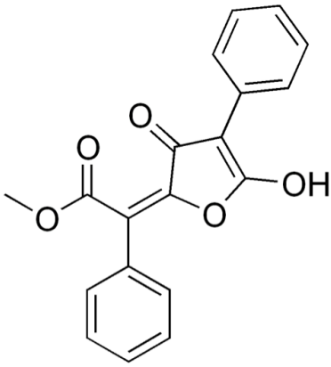
Figure 1. The structure of vulpinic acid.
