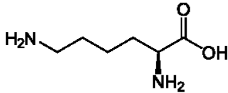
2x L-lysine
