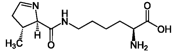
Pyrrolysin
