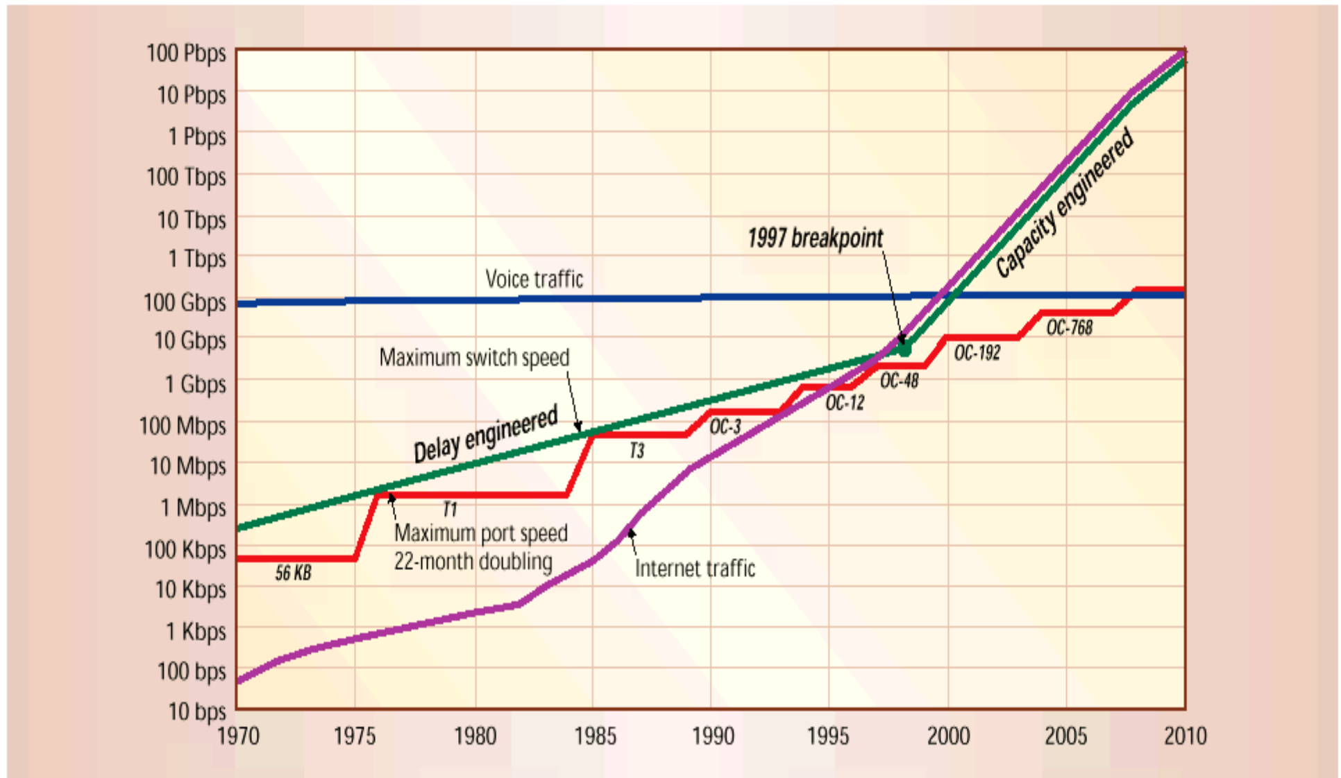
Figure 1. Growth trends for Internet traffic, voice traffic, maximum trunk speed, and maximum switch speed required for large cities. A major breakpoint occurred in 1997, when routers were forced to become wire speed and increase in capacity as fast as Internet traffic growth.
