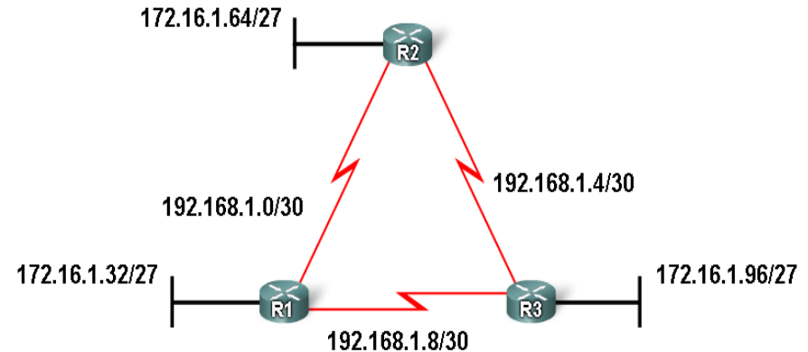
Classless: Subnet mask can vary in the topology
