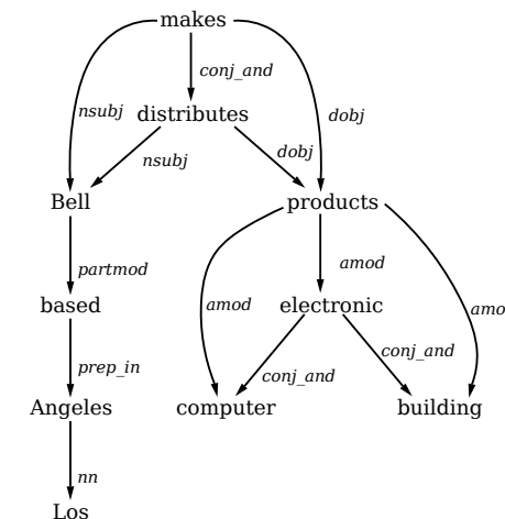
Graphical representation of the SD for the sentence
