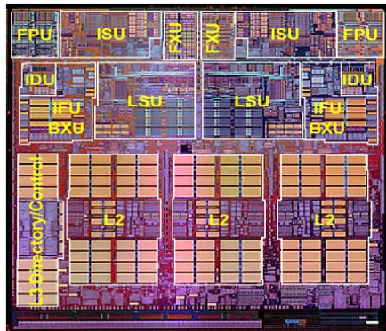
POWER4 Core
