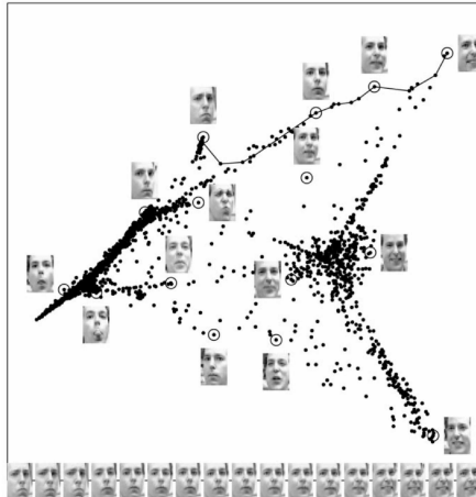
Fig. 3. Images of faces (171) mapped into the embedding space described by the first two coordinates of LLE. Representative faces are shown next to circled points in different parts of the space. The bottom images correspond to points along the top-right path (linked by solid line)
