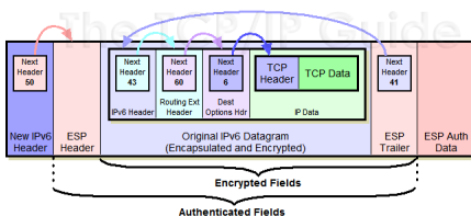
IPv6 ESP Datagram Format - IPsec Tunnel Mode
