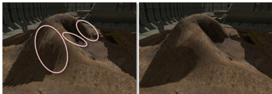
Projective aliasing
