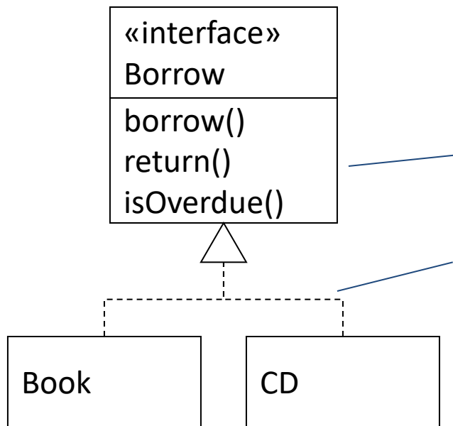
“Class” style notation
