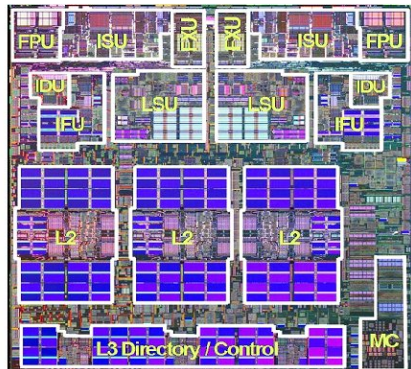
POWER5 Core
