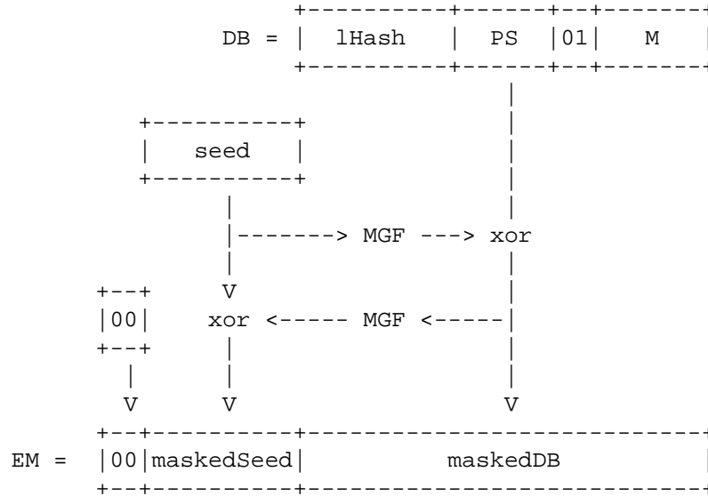
Figure 1: EME-OAEP Encoding Operation
