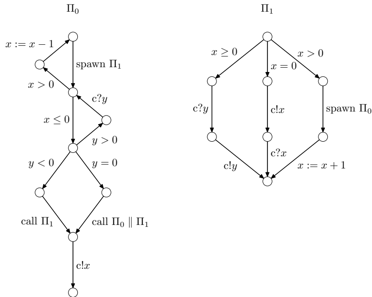
Fig. 8. A flow-graph
