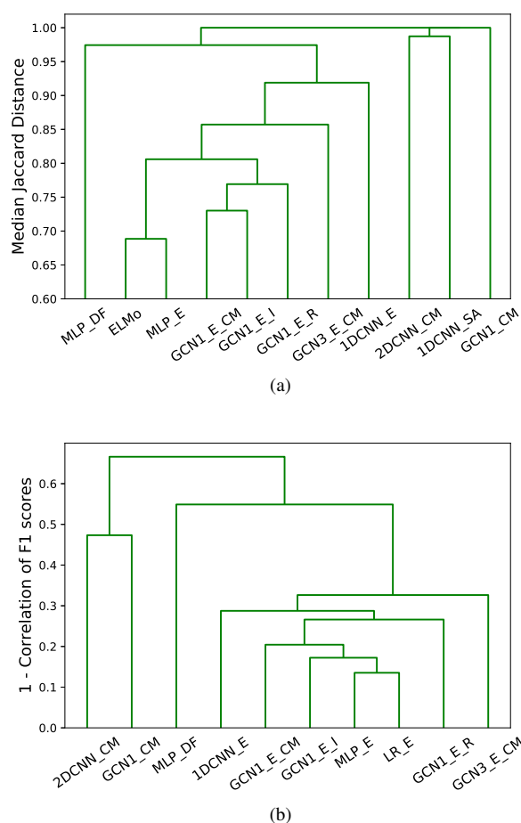
Fig. 3. Hierarchical clustering of the models based on the similarity of the 40 nearest neighbors of each protein in the embedding space (a) and the correlation in protein-centric F_{max} (b).
