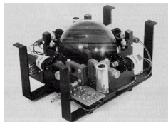
Prototyp trackballu (1952)
