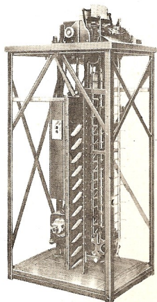
Vertical Sorter
