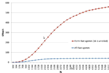
Obrázek: SGEMM optimized for Fermi and Cypress, running on Fermi 1
