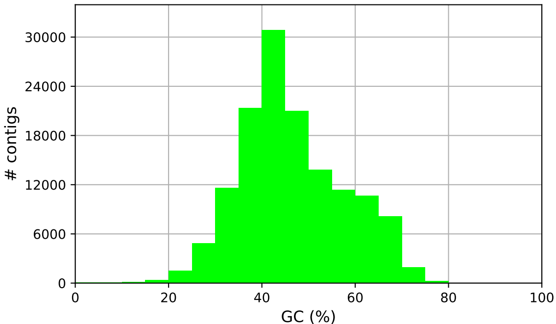
FAQ28413.unclassified GC content
