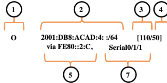
IPv6 Routing Table
