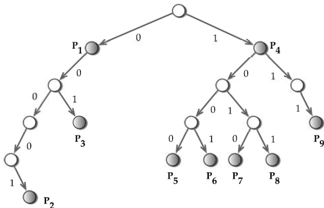
Figure: Binary trie data structure example.
