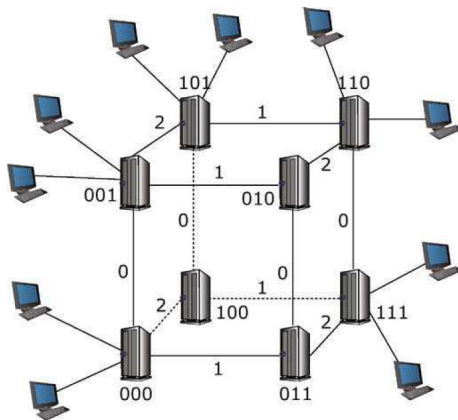
Figure: The Edutella network structure. A query routing in Edutella is first directed to superpeers in HyperCuP network (= HyperCube P2P network), where the suffix-based routing scheme could be employed.
