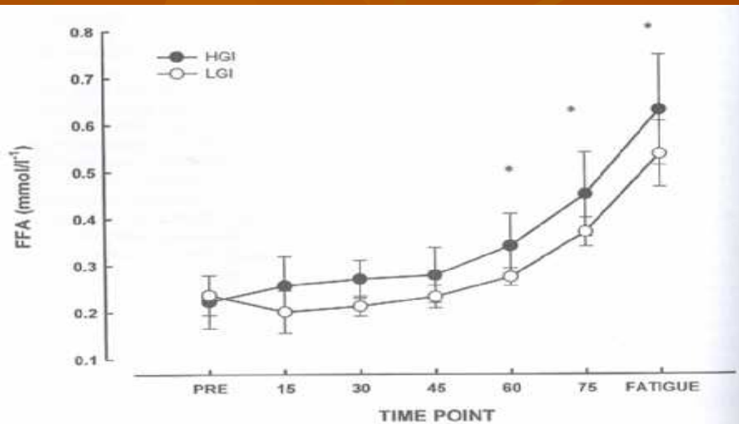
Figure 1 — Plasma FFA concentrations (mmol/L) during R2 in the HGI and LGI trials (mean \pm standard error of the mean). P \leq 0.05 * different from pre-exercise for both groups.
