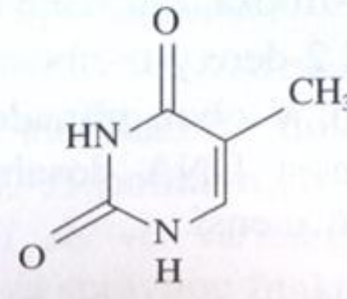
thymin
