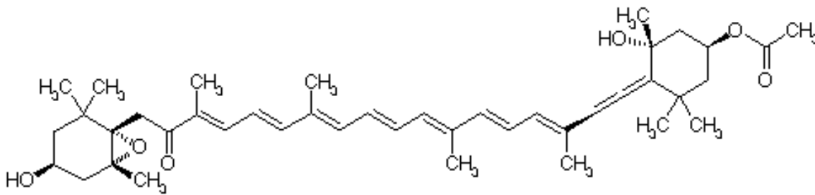
fukoxanthin
