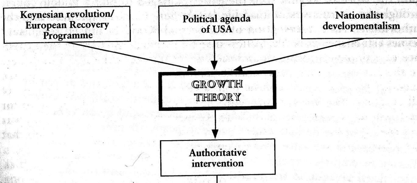
Figure 10 Growth theory
