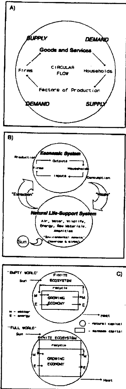
FIG. 2. Schematic depictions of the economic and environmental systems and their relationships. (A) The economy as an isolated system. (B) Linking the economic and environmental systems. (Modified from Tietenberg 1992.) (C) The economy as dependent on the environment.
