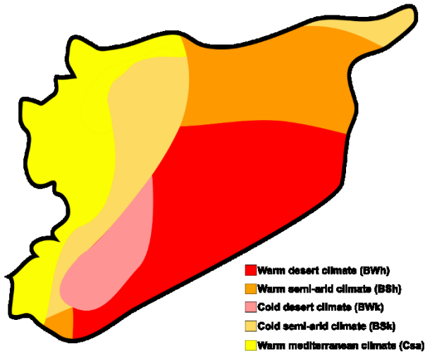
Syria map of Köppen climate classification
