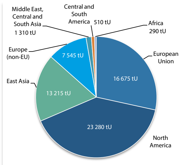
Figure 2.2. World uranium requirements: 62 825 tU (as of 1 January 2017)
