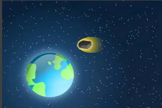
Near-Earth Objects
