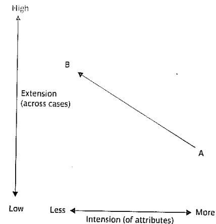
Fig. 2.2 Cartier's ladder of cases
