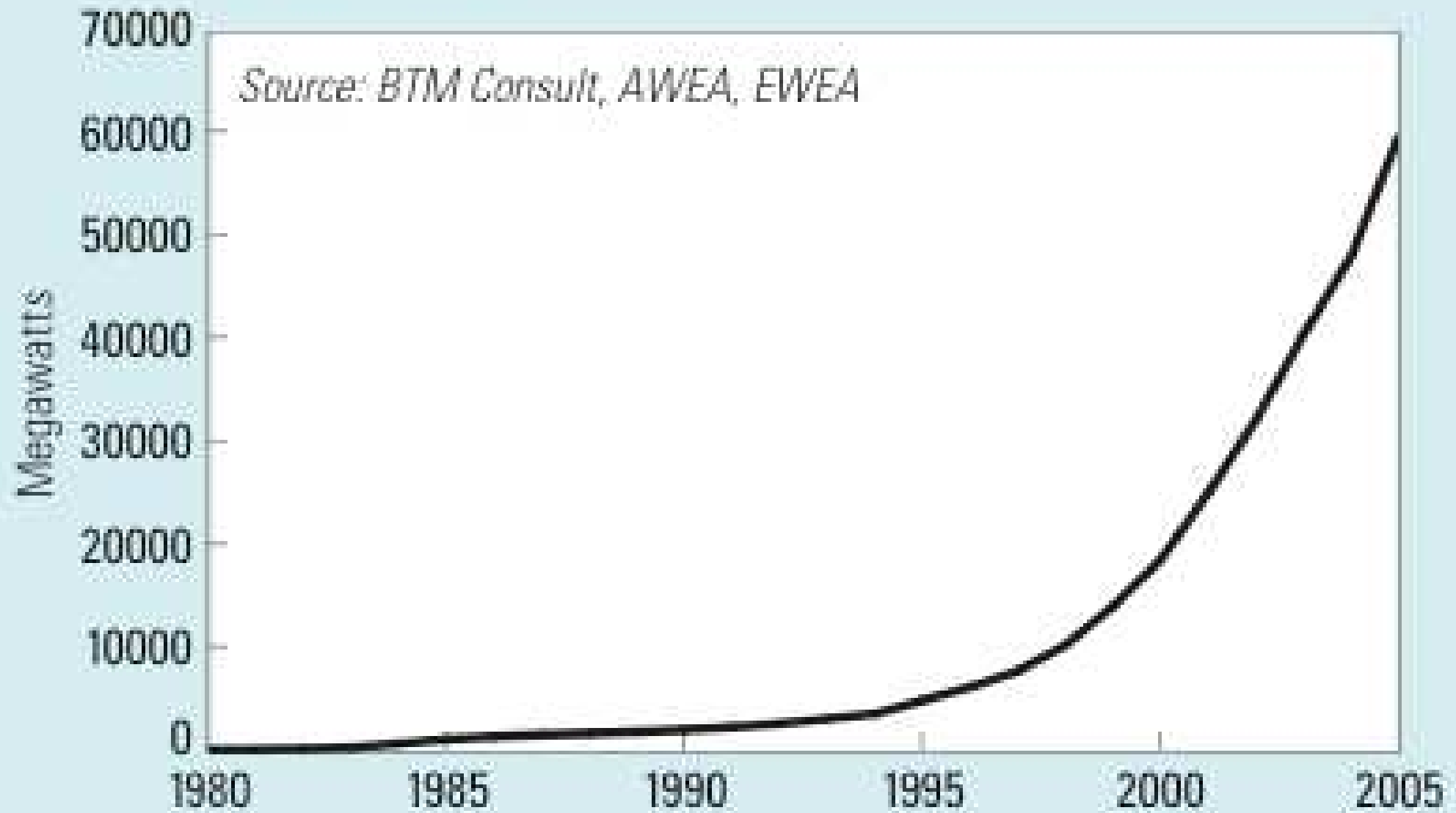
Figure 1. World Wind Energy Generating Capacity, 1980–2005
