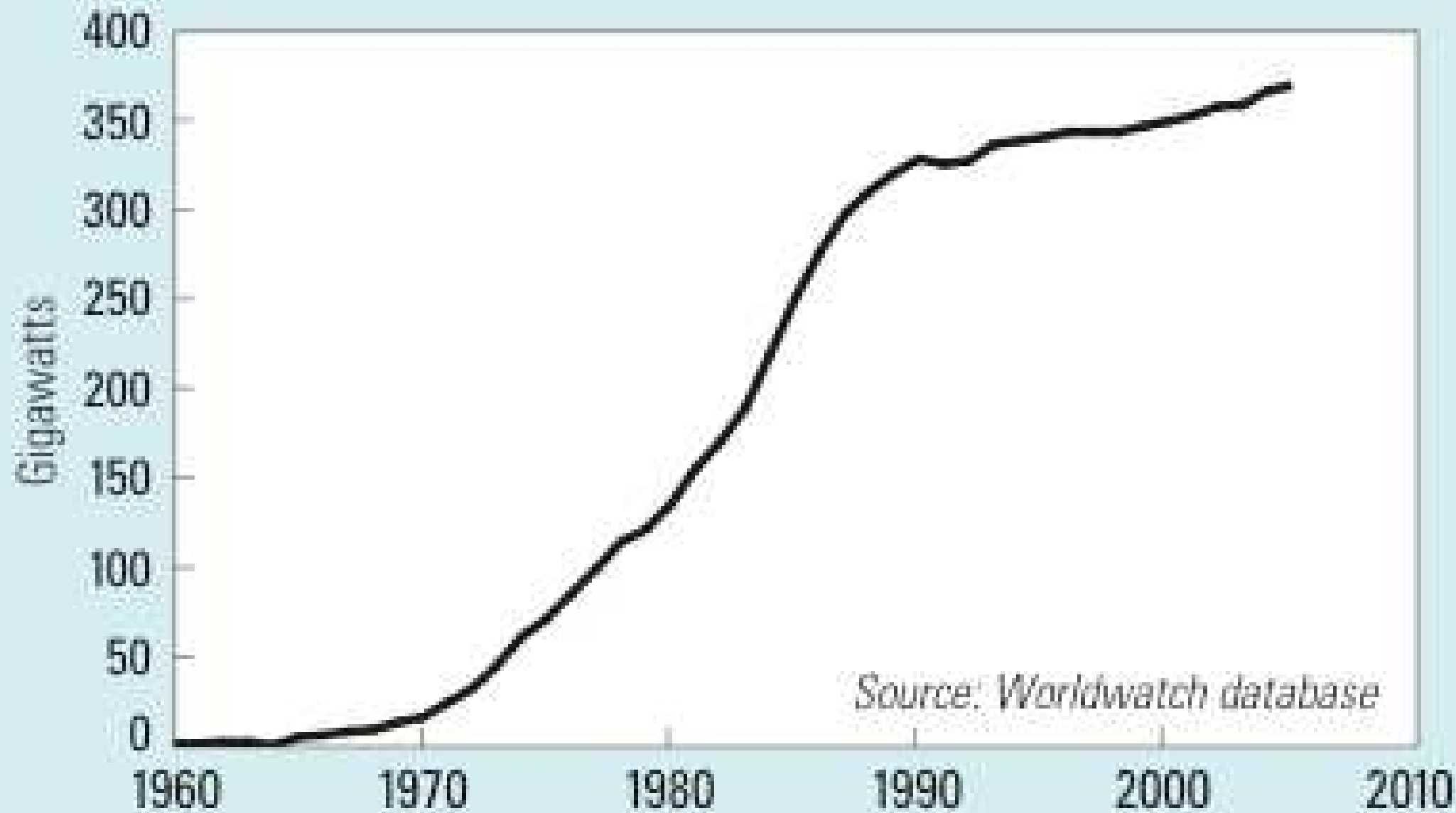
Figure 1. World Electrical Generating Capacity of Nuclear Power Plants, 1960–2005
